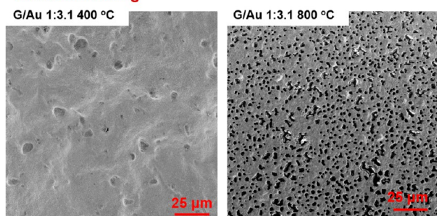
Figure 3. SEM images of the exterior of the sample G/Au = 1:3.1 upon two-step annealing and direct annealing at 400 and 800 °C.
